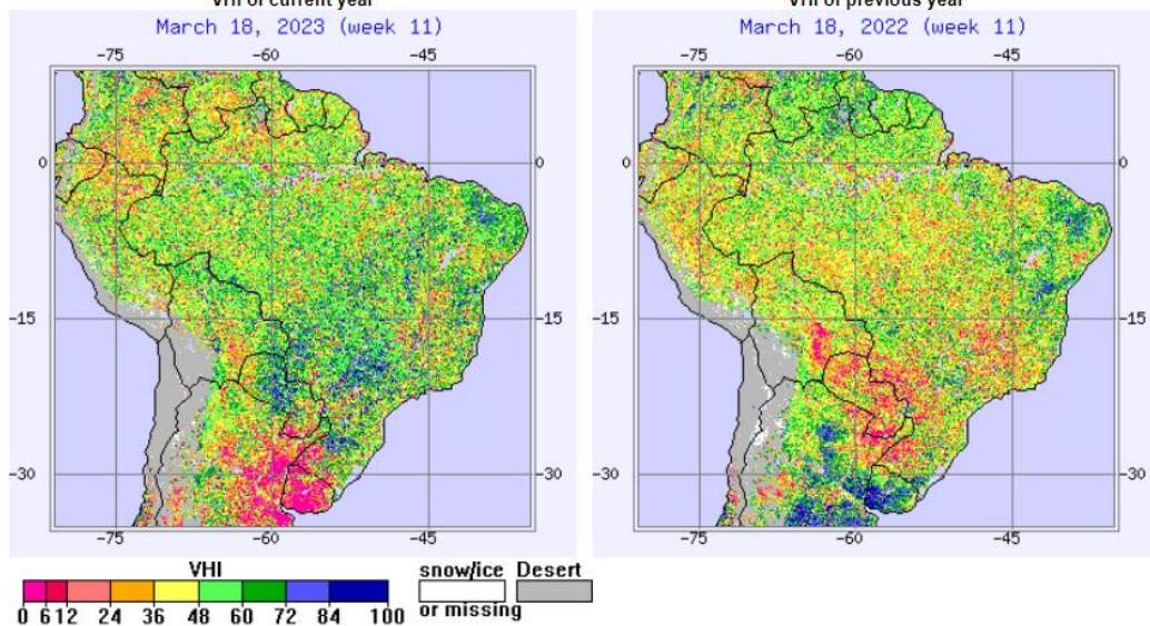
Brazil - Vegetation Health Index (VHI): Current Week and One Year Ago, 2023 week 11
